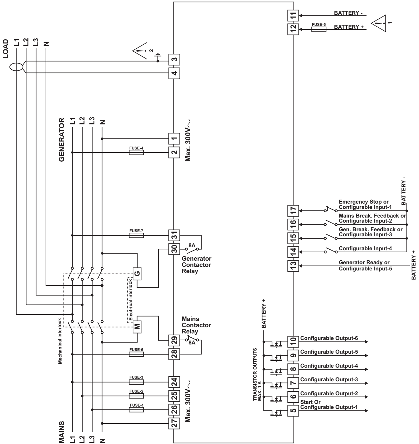
TRANS-MINIATS three phase connections schematic
